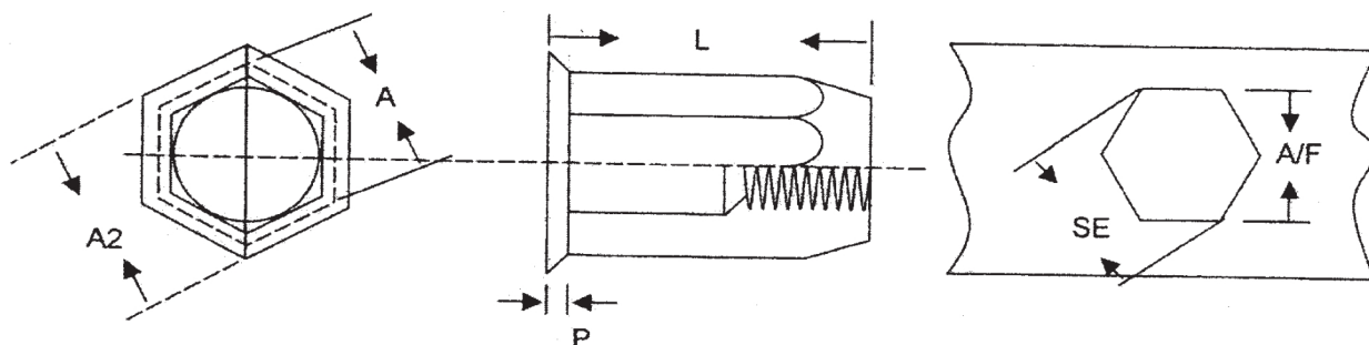
METRIC DIMENSION (mm)
