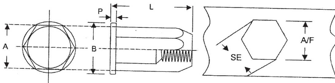
METRIC DIMENSION (mm)
